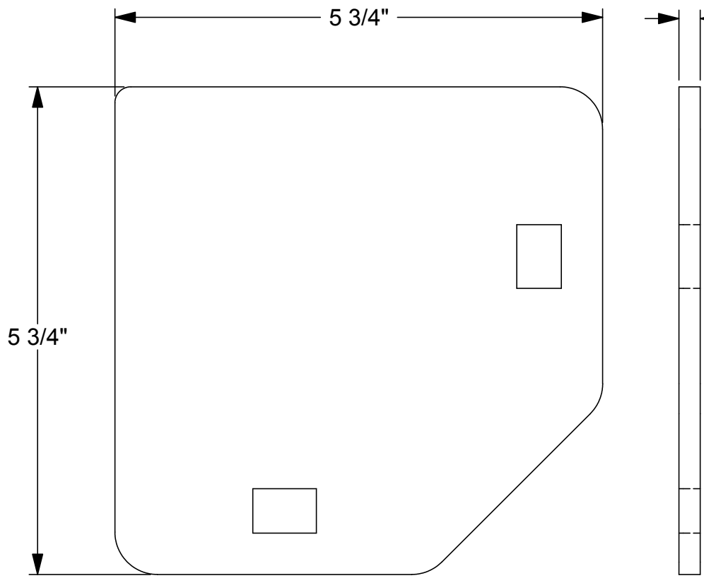
PART # LEG PAD MATERIAL: 1/4" THICK CARBON STEEL QUANTITY: 4
